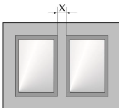
Dubbelmontage X = 100mm
